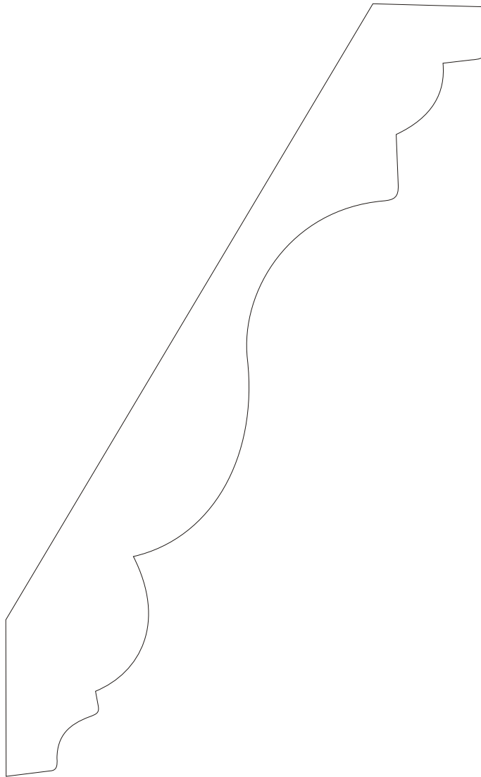
WL35849-S 15/16 x 6-11/16 crown Copyright Flex Trim, Inc. 2005
