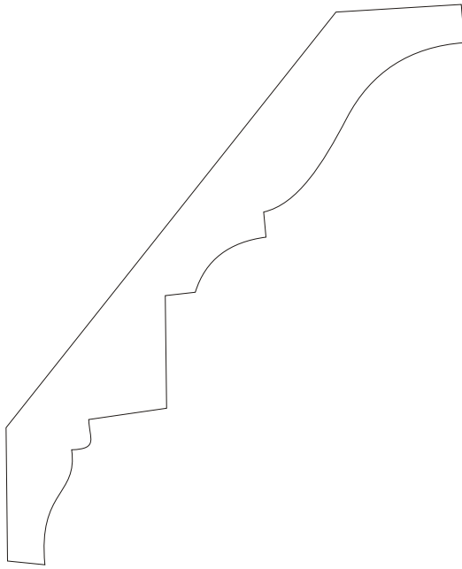
T0340-P 11/16 x 4-1/4 crown Copyright Flex Trim, Inc. 2005
