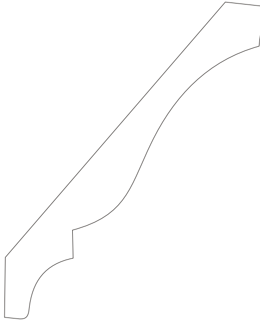
T0320-P 9/16 x 4-1/4 crown Copyright Flex Trim, Inc. 2005
