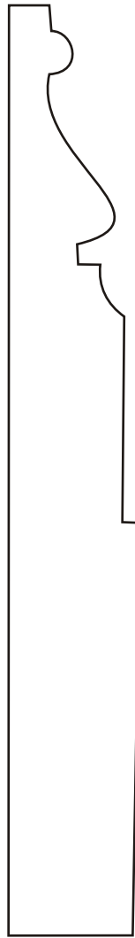
SD696-S 11/16 X 5-1/2 BASE
