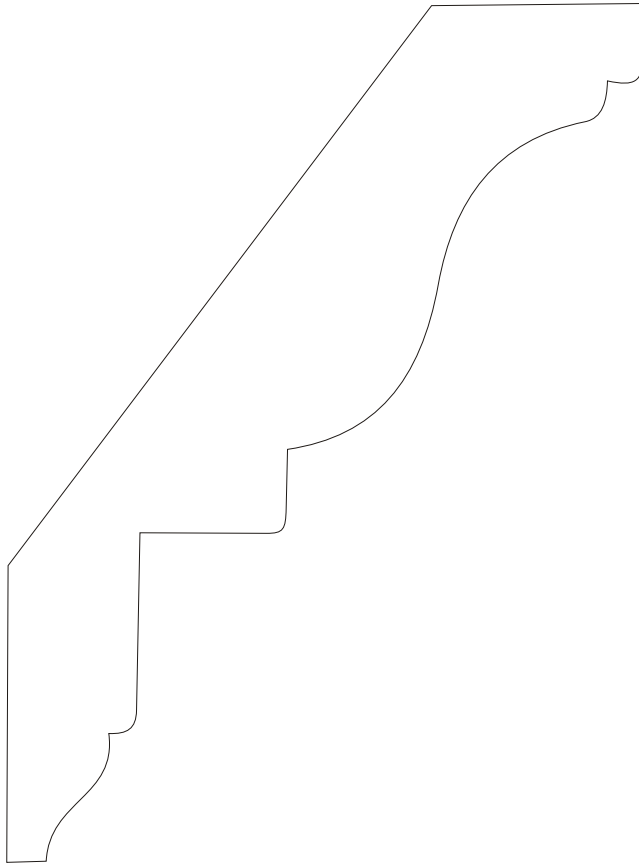
RB7-S 1-1/16 x 5-9/16 crown Copyright Flex Trim, Inc. 2005
