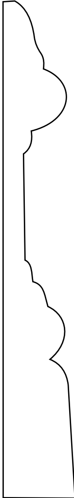
p945-o 3/4 x 5-1/4 base
