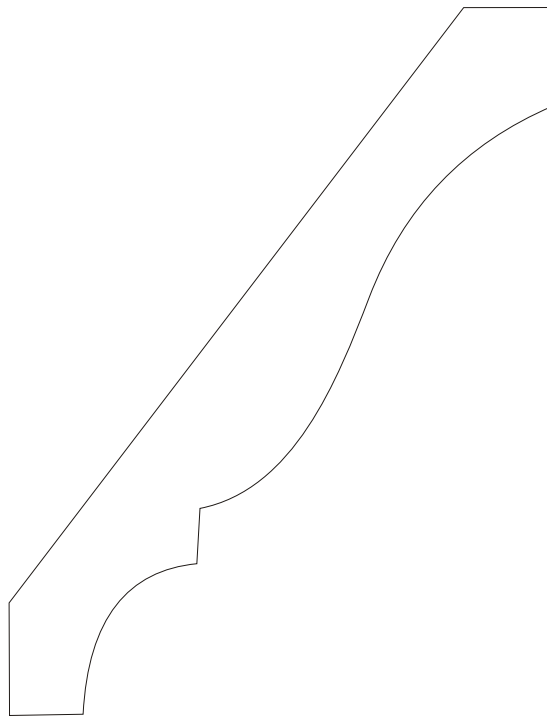
OR047P-S 9/16 x 4-5/8 crown Copyright Flex Trim, Inc. 2006
