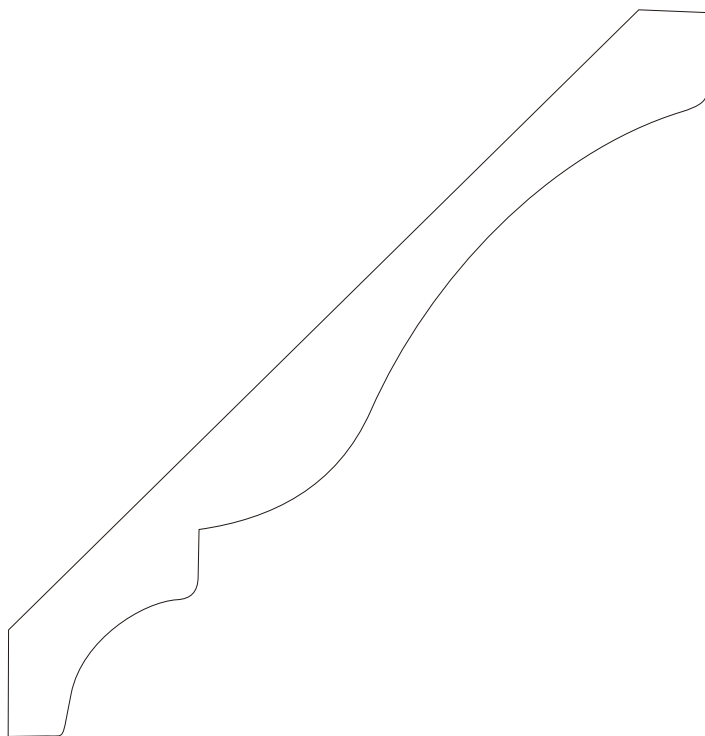
OP555MDF-S 9/16 x 5-1/4 crown Copyright Flex Trim, Inc. 2005
