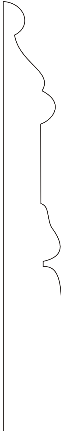
NH750-s 1-1/8 x 7-1/2 Casing 1 x 7-3/8(measured)
