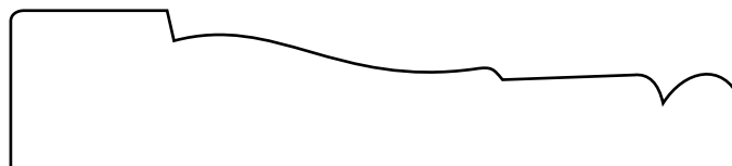
MWN13 ~ smooth 3/4 x 3-1/2 CASING
