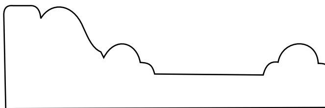
MMSM3 ~ smooth 1-1/16 x 3-3/8 CASING
