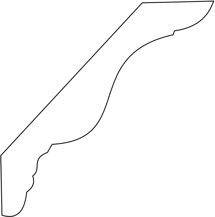
MH408-o 3/4 x 5 Crown 13/16 x 5 (measured)
