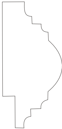
KMMWS214CR-F 1-1/8 x 2-1/4 chair rail Copyright Flex Trim, Inc. 2007
