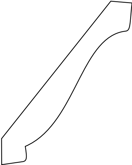
kcp492-smooth/pine 9/16 x 3-1/2 crown
