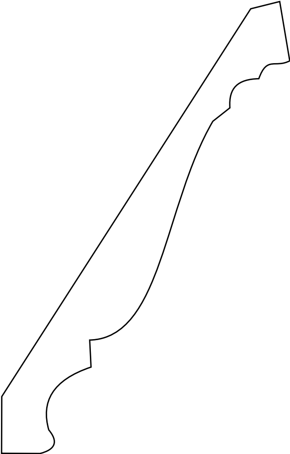
JT558-s 5/8 x 5-5/8 Crown 5/8 x 5-1/2 (measured)
