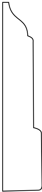
JPM02 ~ smooth/pine 5/8 x 3-1/4 BASE
