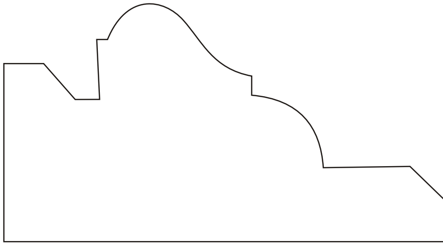
HP475-s 2-1/2 x 4-5/8 Casing
