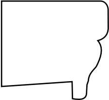
hm436-s 1-1/16 x 1-1/4 curved (bull nose)
