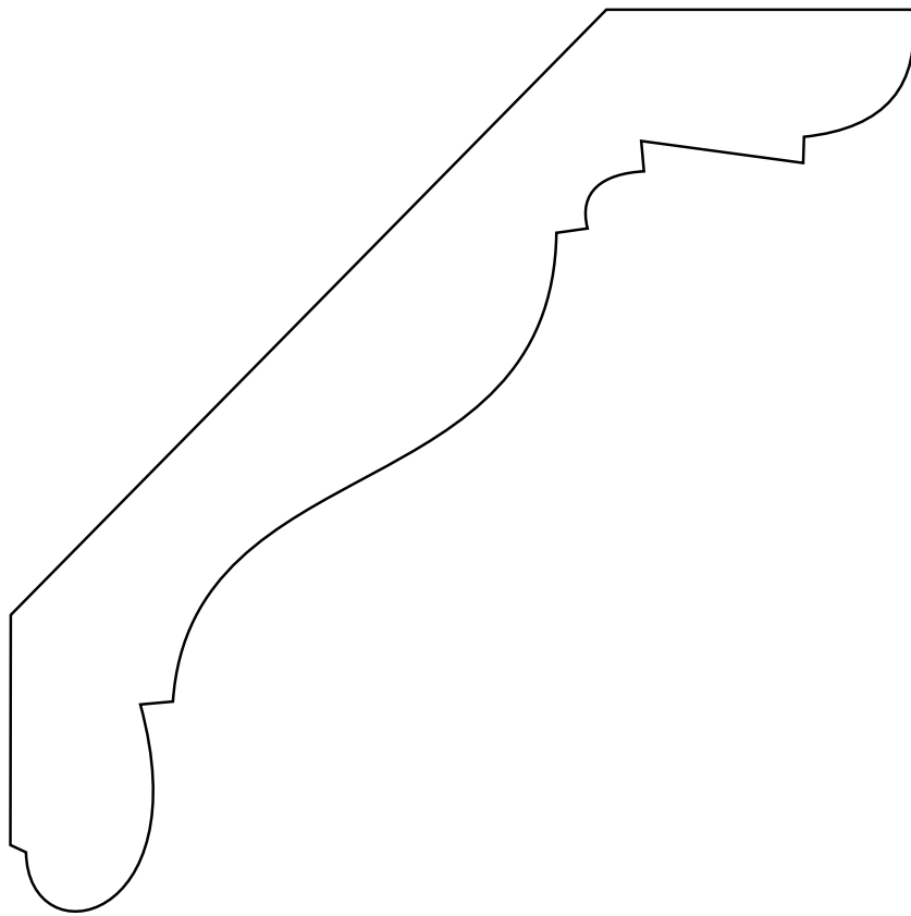
HLGIS-s 1-1/4 x 6 Crown 7/8 x 5-7/8(measured)
