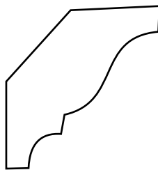
HLO74 ~ smooth 9/16 x 1-5/8 CROWN
