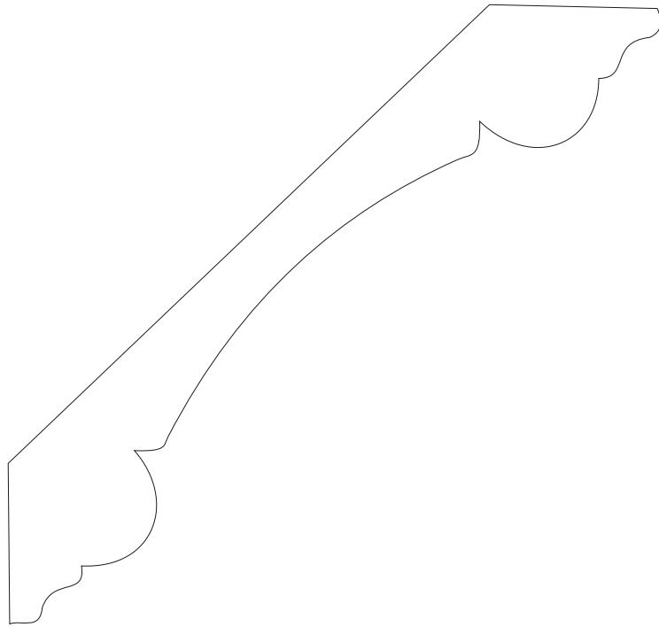
GG-1-S 7/8 x 5-3/16 crown Copyright Flex Trim, Inc. 2005
