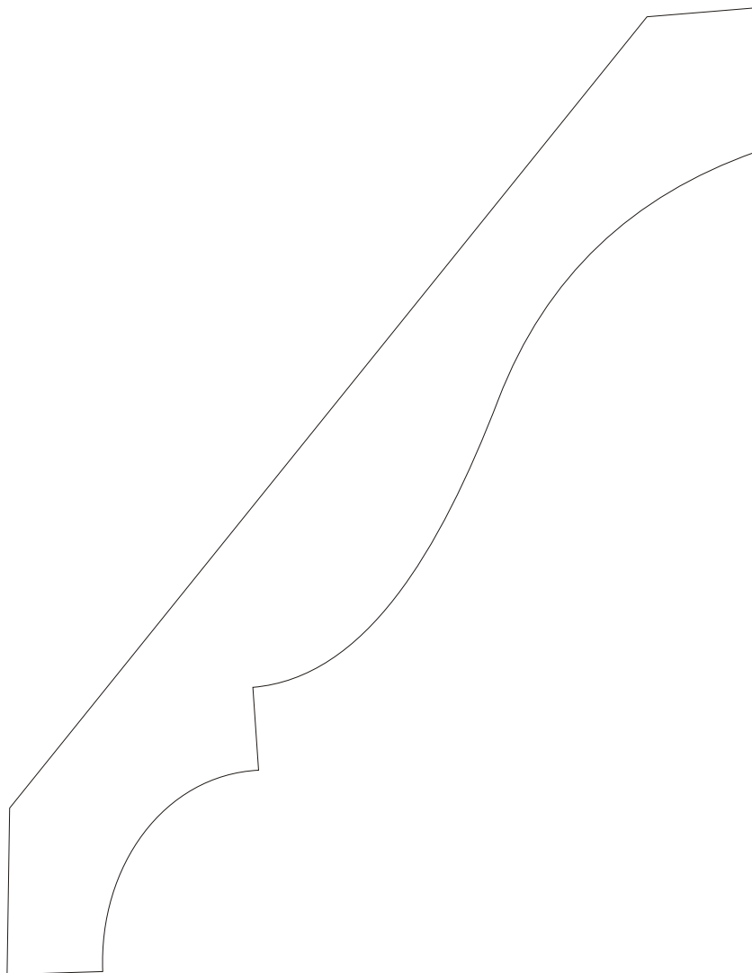
ECP41-S 1 x 7-1/16 crown Copyright Flex Trim, Inc. 2005
