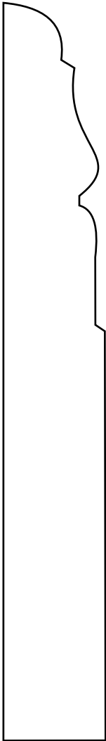
CW362 ~ smooth 3/4 x 5-1/2 BASE
