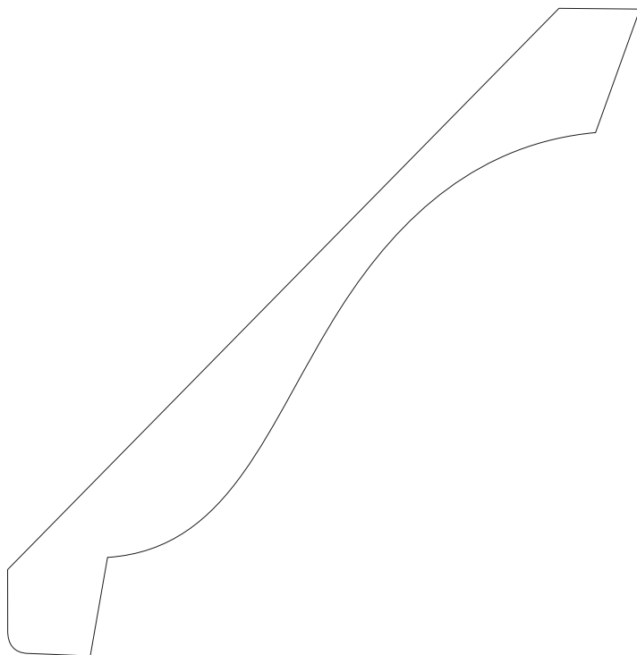
BW8004-S 11/16 x 5-1/4 crown Copyright Flex Trim, Inc. 2005
