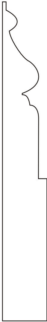
AG149-s 3/4 x 5-1/2 Base
