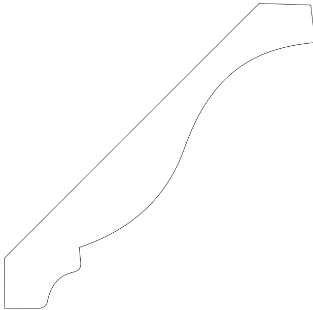
AC039-S 11/16 x 4-7/16 crown Copyright Flex Trim, Inc. 2005
