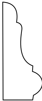
WBH002 ~ smooth 11/16 x 1-7/8 BASE CAP
