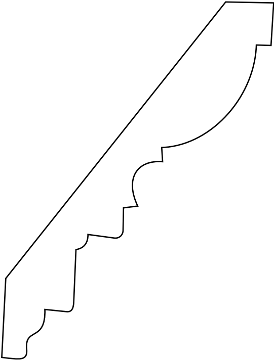
FM-CR622 ~ oak 3/4 x 4-1/2 CROWN
