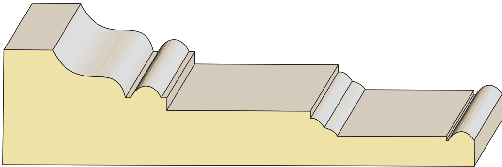
CL-358-L Casing 1 1/4 X 5-1/16
