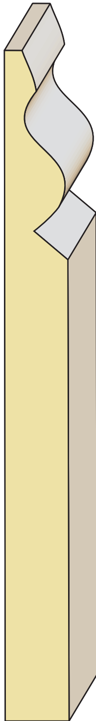
BA718 Base 11/16 X 7-1/8
