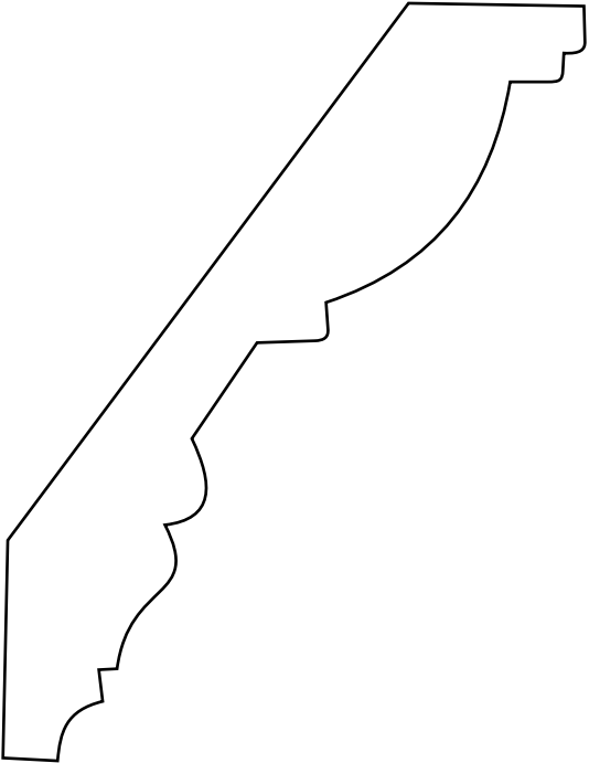
ABJAN4 ~ smooth 13/16 x 4-1/2 CROWN
